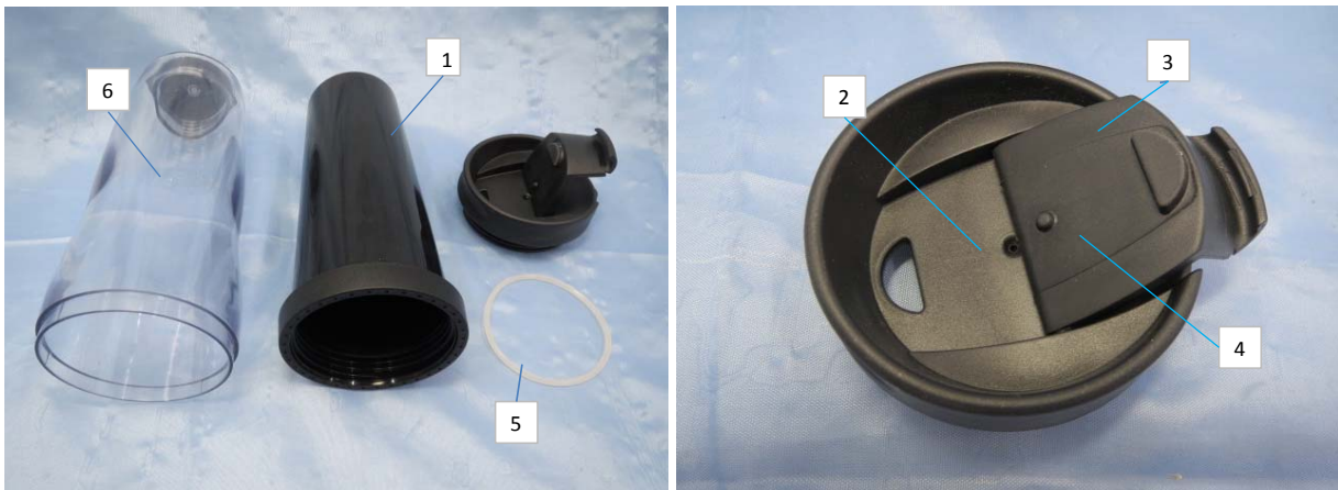
Development view
